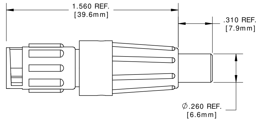
ASSEMBLED KIT VIEW FOR CUSTOMER REFERENCE
