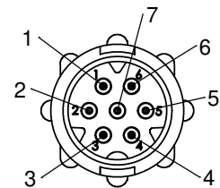
FACE VIEW 18982-7PG-5XX 7 POSITION A-KEY
