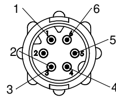
FACE VIEW 18982-6PG-5XX 6 POSITION B-KEY
