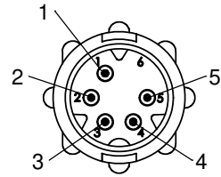
FACE VIEW 18982-5PG-5XX 5 POSITION A-KEY
