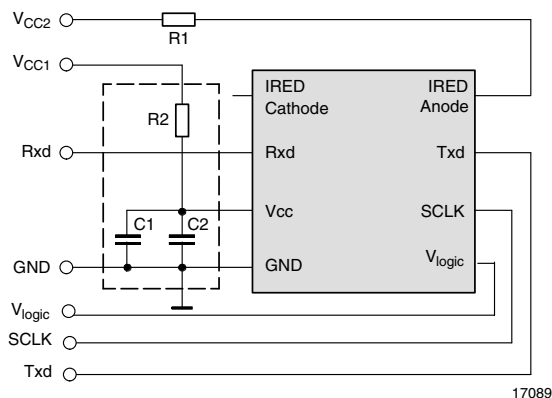
Figure 3. Recommended Application Circuit All external components (R, C) are optional
