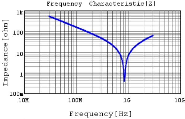
RCE5C1H100J0A2H03B |Z| DC0V, 25degC
