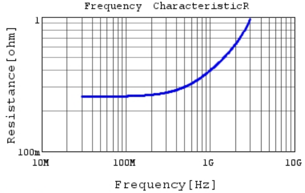
RCE5C1H100J0A2H03B R DC0V, 25degC
