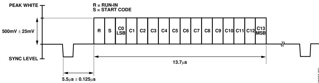
Figure 93. PS 625p CGMS-A Waveform (Line 43)
