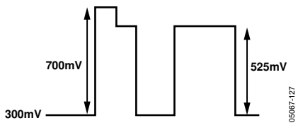
Figure 127. PS RGB Output Levels
