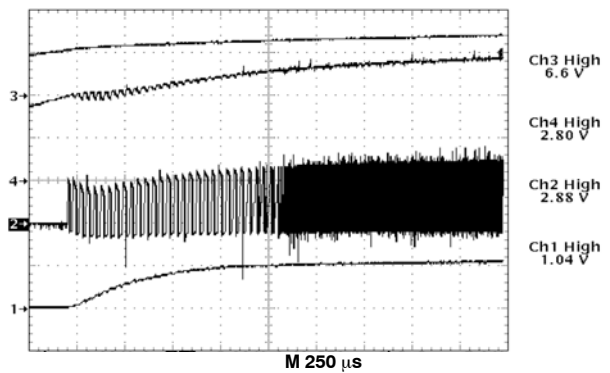
Trace 1– Regulator Output Voltage (1.0 V/div.) Trace 2– Inductor Switching Node (2.0 V/div.) Trace 3– 12 V Input ( V_{\text{CC}} ) (5.0 V/div.) Trace 4– 5.0 V Input (1.0 V/div.)
