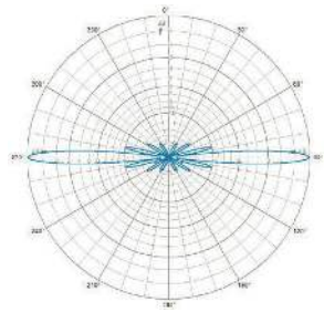
E-Plane | 405 MHz
