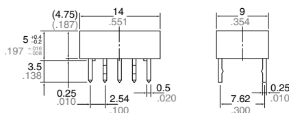
Self-clinching terminal
