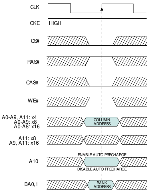
Figure 5 READ Command
