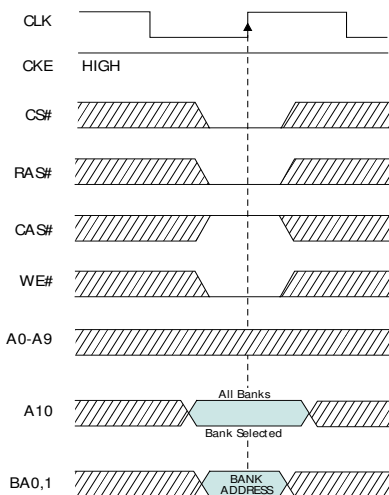
Figure 20 PRECHARGE Command
