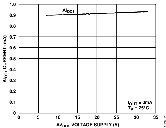
Figure 71. A_{LDD1} Current vs. A_{VDD1} Voltage Supply
