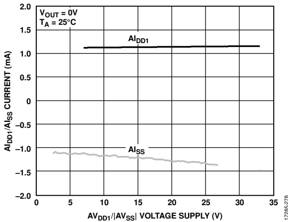
Figure 70. A_{LDD1}/A_{LSS} Current vs. A_{VDD1}/A_{VSS} Voltage Supply
