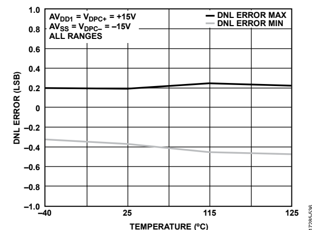
Figure 36. DNL Error vs. Temperature
