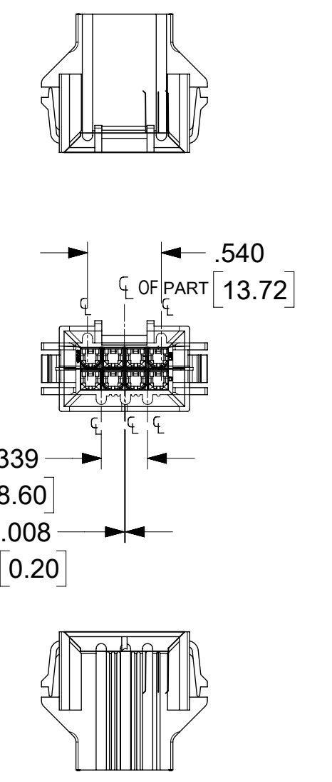
8 CIRCUIT
