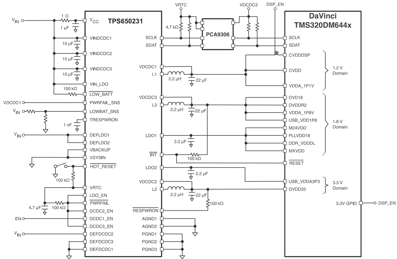
Figure 42. Typical Configuration for the Texas Instruments TMS320DM644x DaVinci Processors
