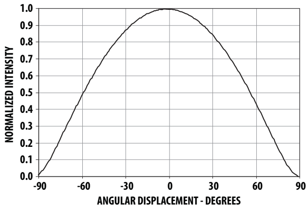
Figure 10. Radiation Pattern
