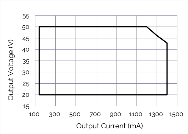
Figure 3: Operating Window
