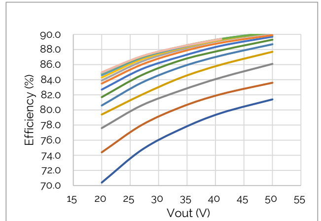
Figure 9: Efficiency @ 277VAC
