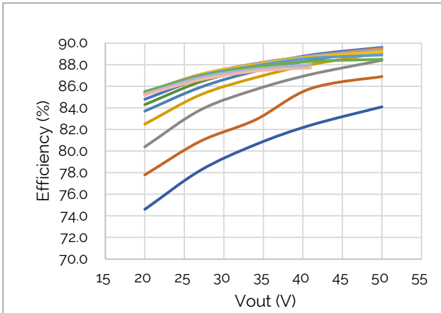
Figure 8: Efficiency @ 120VAC
