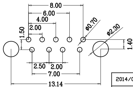
RECOMMENDED PCB LAYOUT TOLERANCE: ±0.05mm
