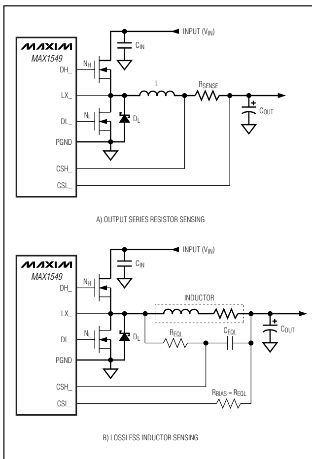
Figure 8. Current-Sense Configurations
