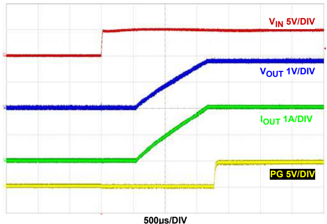
FIGURE 39. START-UP V IN AT 2A LOAD, V IN = 5V, MODE = PWM, T A = +25°C
