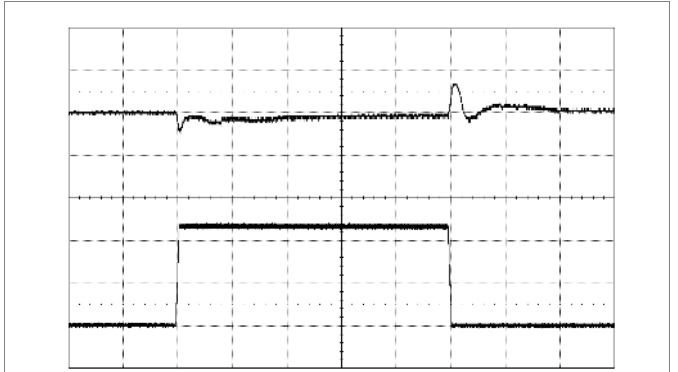
Output voltage response to load Step-change (6.25-18.75-6.25 A) at: T_{P1} = +25 °C, V_I = 12 V, V_O = 1.0 V di/dt = 2 A/ \mu s, f_{sw} = 320 kHz C_O = 470 \mu F/10 m \Omega Top trace: output voltage (200 mV/div.). Bottom trace: load current (5 A/div.). Time scale: (0.1 ms/div.)
