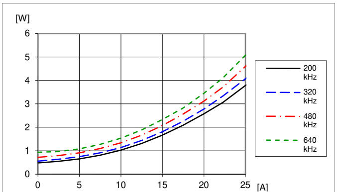
Dissipated power vs. load current and switch frequency at T_{P1} = +25 \text{ }^\circ\text{C} , V_I = 12 \text{ V} , V_O = 1.0 \text{ V} , C_O = 470 \text{ }\mu\text{F}/10 \text{ m}\Omega . Default configuration except changed frequency
