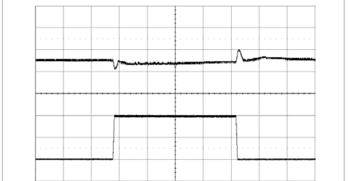
Output voltage response to load current step-change (5-15-5 A) at: T_{P1} = +25\text{ }^\circ\text{C} , V_I = 12\text{ V} , V_O = 1.0\text{ V} , di/dt = 2\text{ A}/\mu\text{s} , f_{sw} = 320\text{ kHz} , C_O = 470\text{ }\mu\text{F}/10\text{ m}\Omega
