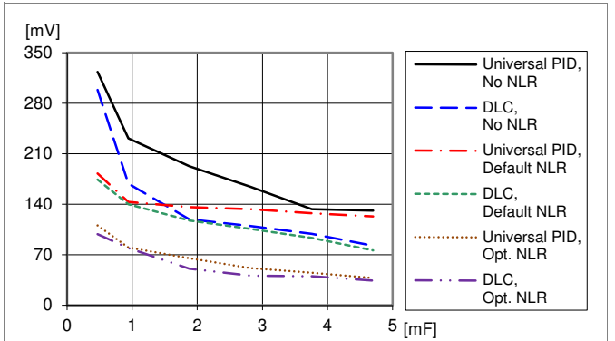
Load transient peak voltage deviation vs. external capacitance. Step (6.25-18.75-6.25 A). Parallel coupling of capacitors with 470 \mu F/10 m \Omega , T_{P1} = +25 °C. V_I = 12 V, V_O = 3.3 V, f_{sw} = 320 kHz, di/dt = 2 A/ \mu s
