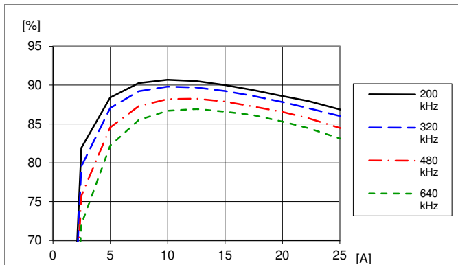
Efficiency vs. load current and switch frequency at T_{P1} = +25 \text{ }^\circ\text{C} , V_I = 12 \text{ V} , V_O = 1.0 \text{ V} , C_O = 470 \text{ }\mu\text{F}/10 \text{ m}\Omega . Default configuration except changed frequency
