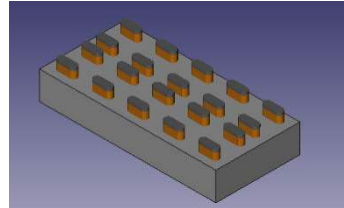
Figure 2. WLCSP, Die Size 2.475mmx1.170mm
