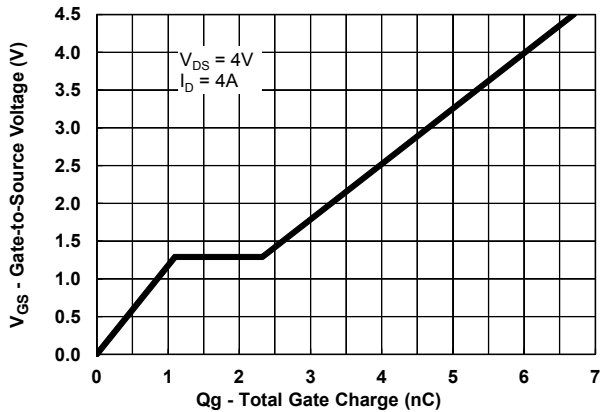
Figure 11. Gate Charge
