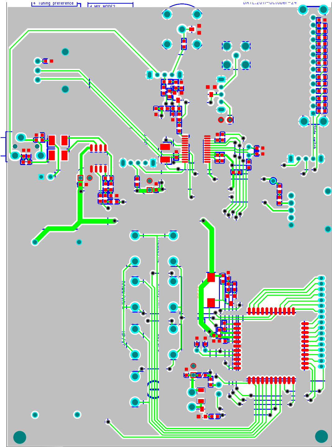
Figure 7. Si4822/26-DEMO Board Gerber Rev 1.0
