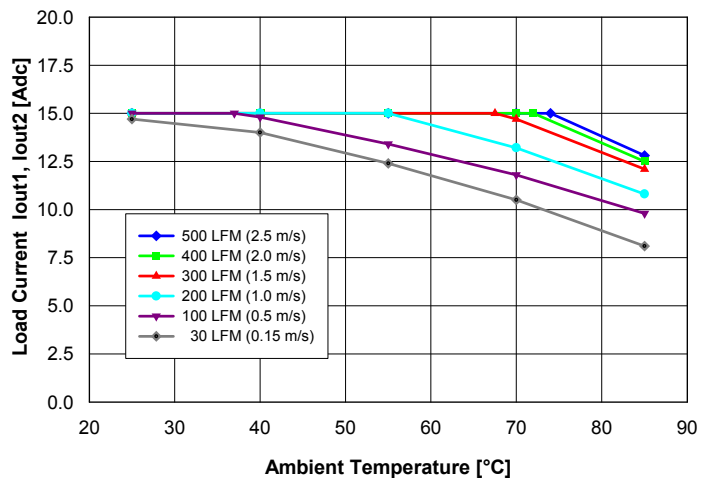
Fig. 11: Available balanced load current (Iout1 = Iout2) vs. ambient temperature and airflow rates for converter mounted with D height pins horizontally with Vin = 48 V, air flowing from pin 3 to pin 1 and maximum FET temperature ≤ 120°C.
