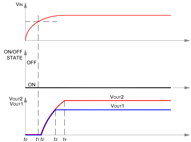
Fig. 5: Start-up scenario #1.
