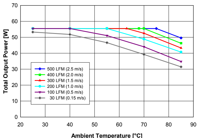
Fig. 1: Available output power vs. ambient air temperature and airflow rates for QD48T012025 converter with D height pins mounted vertically with air flowing from pin 3 to pin 1, MOSFET temperature \leq 120^{\circ}\text{C} , V_{in} = 48\text{ V} and balanced load on both outputs ( I_{out1} = I_{out2} ).
