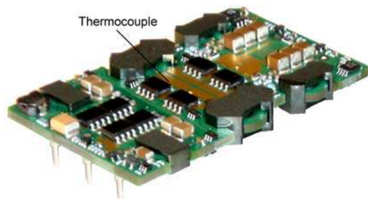
Fig. 34: Location of the thermocouple for thermal testing.
