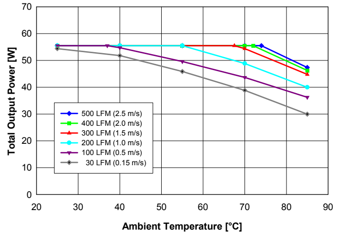
Fig. 9: Available output power for balanced load current (Iout1 = Iout2) vs. ambient air temperature and airflow rates for converter with D height pins mounted horizontally with Vin = 48 V, air flowing from pin 3 to pin 1 and maximum FET temperature ≤ 120°C.
