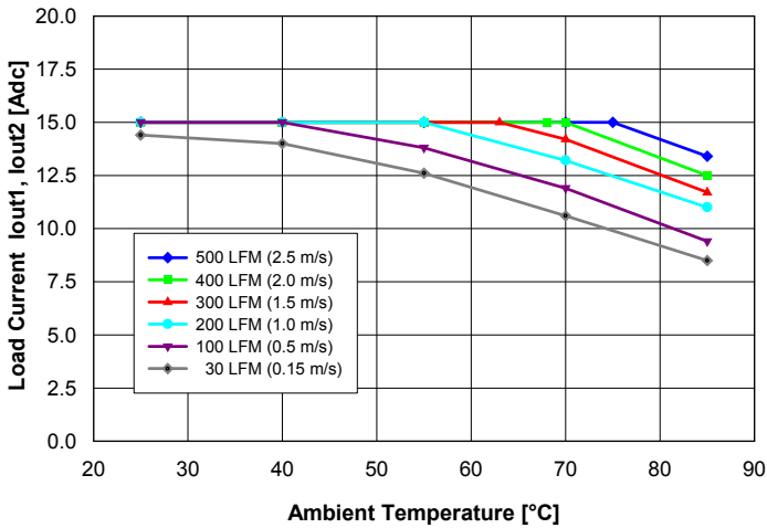
Fig. 10: Available balanced load current (Iout1 = Iout2) vs. ambient air temperature and airflow rates for converter with D height pins mounted vertically with Vin = 48 V, air flowing from pin 3 to pin 1 and maximum FET temperature ≤ 120°C.
