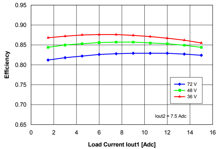
Fig. 13: Efficiency vs. load current Iout1 and input voltage for converter mounted horizontally with air flowing from pin 3 to pin 1 at a rate of 300 LFM (1.5 m/s), for Iout2 = 7.5 A and Ta = 25°C.
