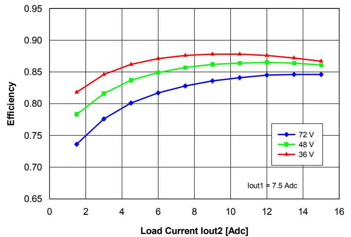
Fig. 15: Efficiency vs. load current Iout2 and input voltage for converter mounted horizontally with air flowing from pin 3 to pin 1 at a rate of 300 LFM (1.5 m/s), for Iout1 = 7.5 A and Ta = 25°C.
