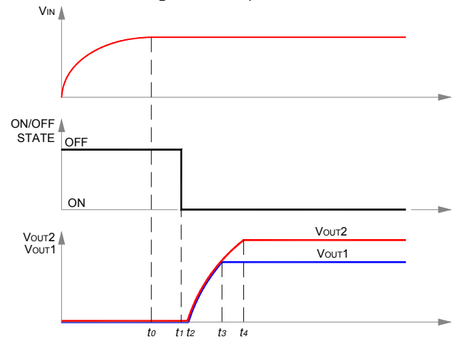
Fig. 6: Start-up scenario #2.
