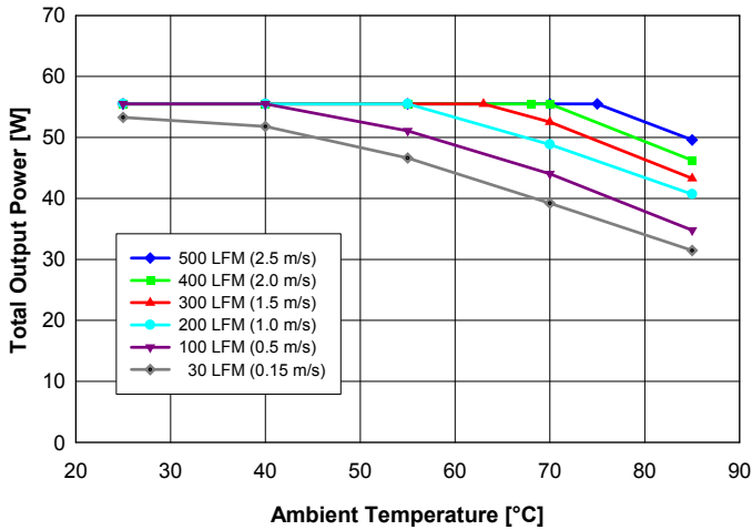
Fig. 8: Available output power for balanced load current (Iout1 = Iout2) vs. ambient air temperature and airflow rates for converter with D height pins mounted vertically with Vin = 48 V, air flowing from pin 3 to pin 1 and maximum FET temperature ≤ 120°C.
