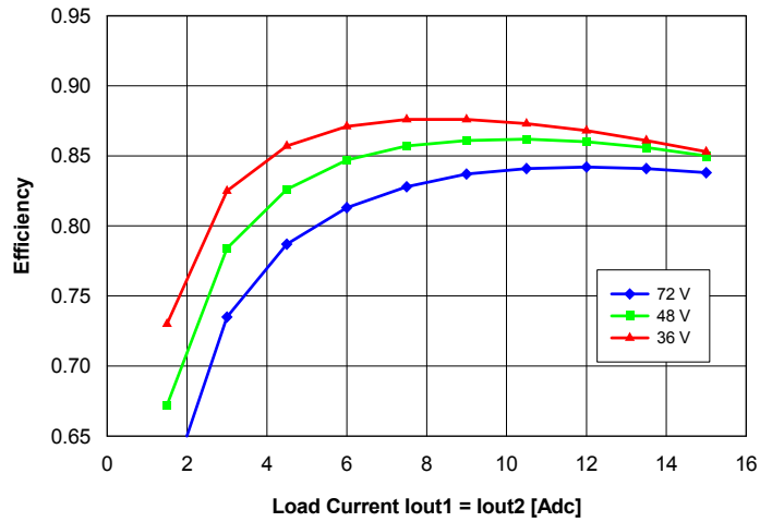
Fig. 17: Efficiency vs. balanced load current ( I_{out1} = I_{out2} ) and input voltage for converter mounted horizontally with air flowing from pin 3 to pin 1 at a rate of 300 LFM (1.5 m/s) and T_a = 25^\circ\text{C} .
