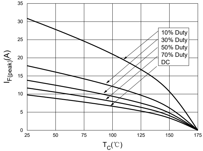
Fig. 7 - Current Derating
