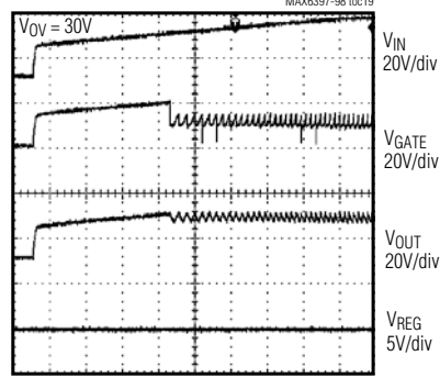
VOLTAGE LIMIT FAULT
