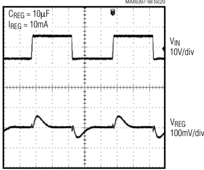
TRANSIENT RESPONSE
