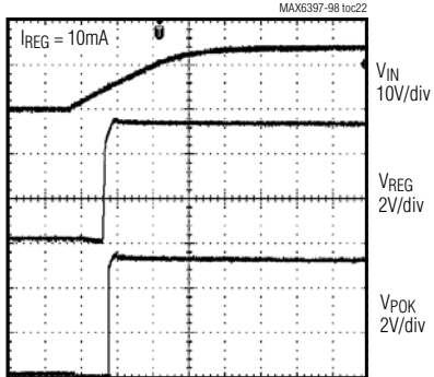
REGULATOR STARTUP WAVEFORM
