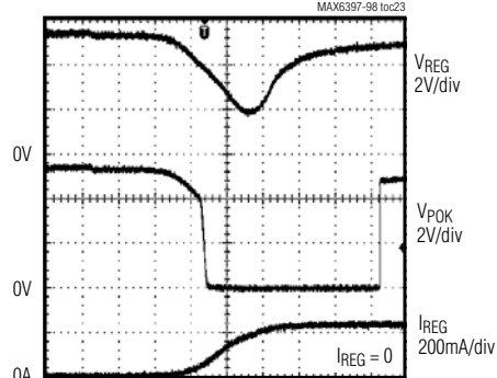
REGULATOR POK ASSERTION
