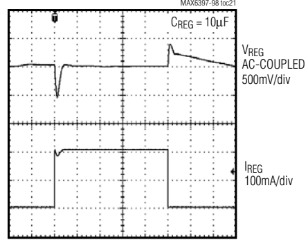
REG LOAD-TRANSIENT RESPONSE
