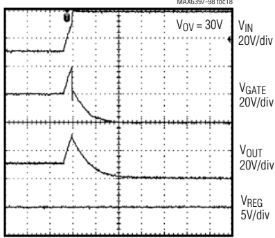
OVERVOLTAGE SWITCH FAULT
