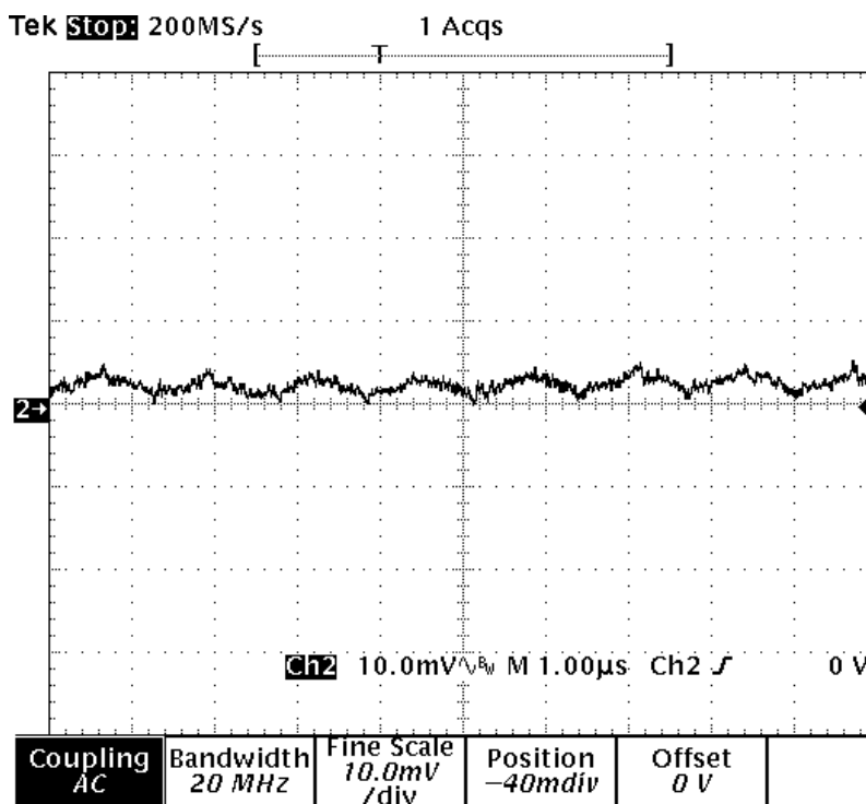
Figure 8. Output Ripple (1.5-V V_{IN} , 0.75-V V_{OUT} , 3-A I_{OUT} , f_{SW} = 600 kHz)
