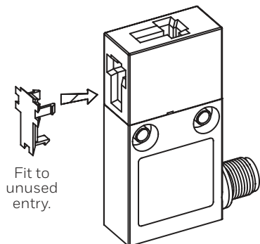
Figure 4. Slot Dust Cover
