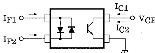
Fig. 8.1 Collector Current Ratio Test Circuit
