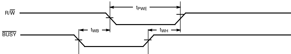
Figure 13. Write Timing with Busy Input (M/ \overline{S} =LOW)
