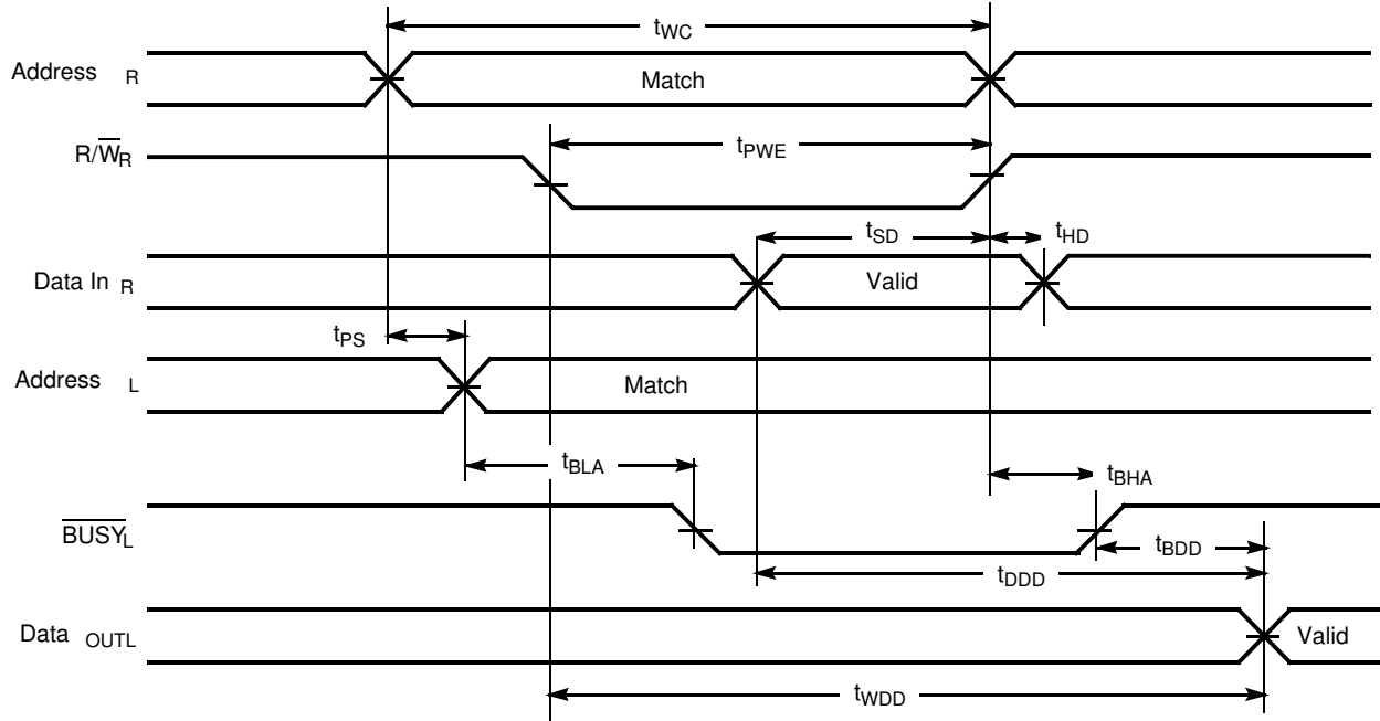
Figure 13. Write Timing with Busy Input (M/ \overline{S} =LOW)
