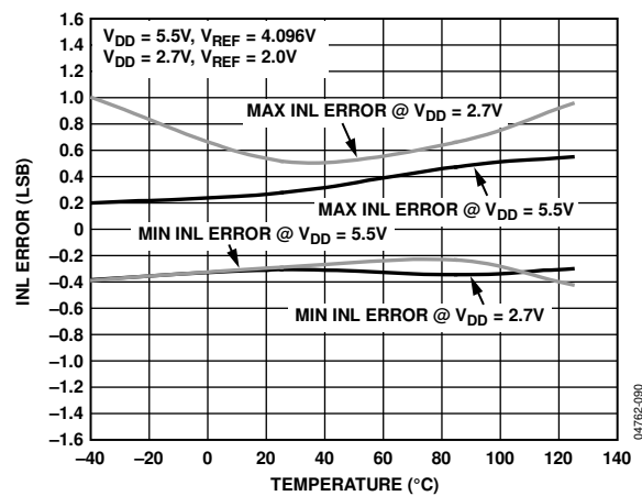
Figure 9. INL vs. Temperature
