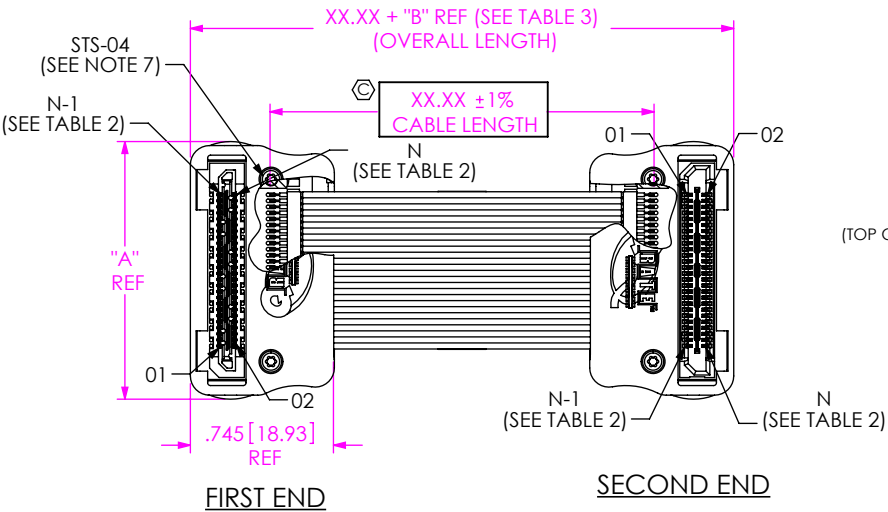
FIG 1 (EQRD-026-XX.XX-TTL-STL-X SHOWN)
