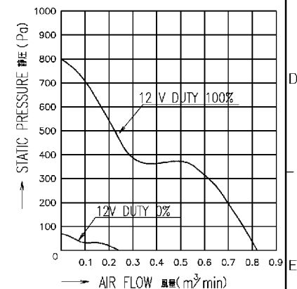
PERFORMANCE CURVES 風量-静圧特性例
