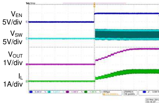
Time 400µs/div
