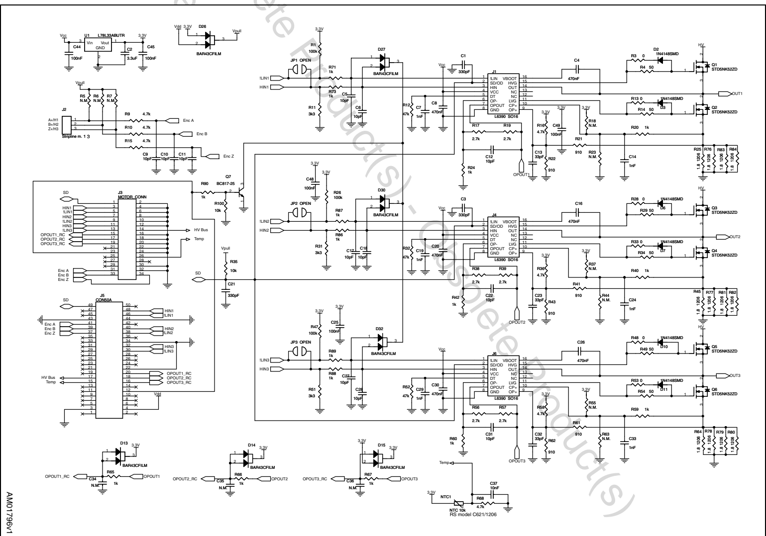
Figure 1. Inverter schematic
