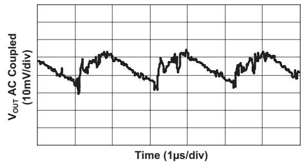
Output Ripple ( I_{OUT} = 100mA ; V_{IN} = 3.0V )
