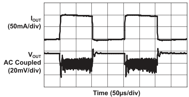
Load Transient Response (V_{IN} = 2.6V)
