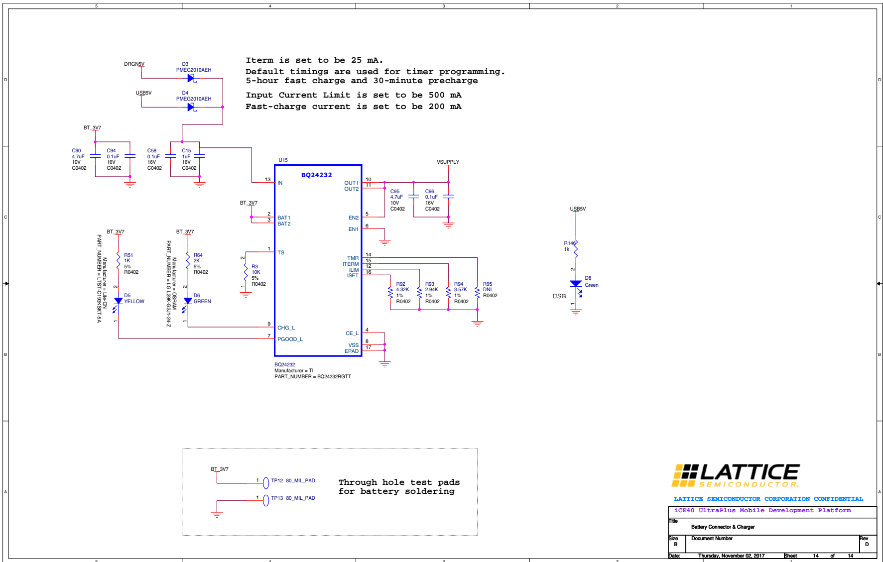
Figure A.14. Battery Connector USB Charger
