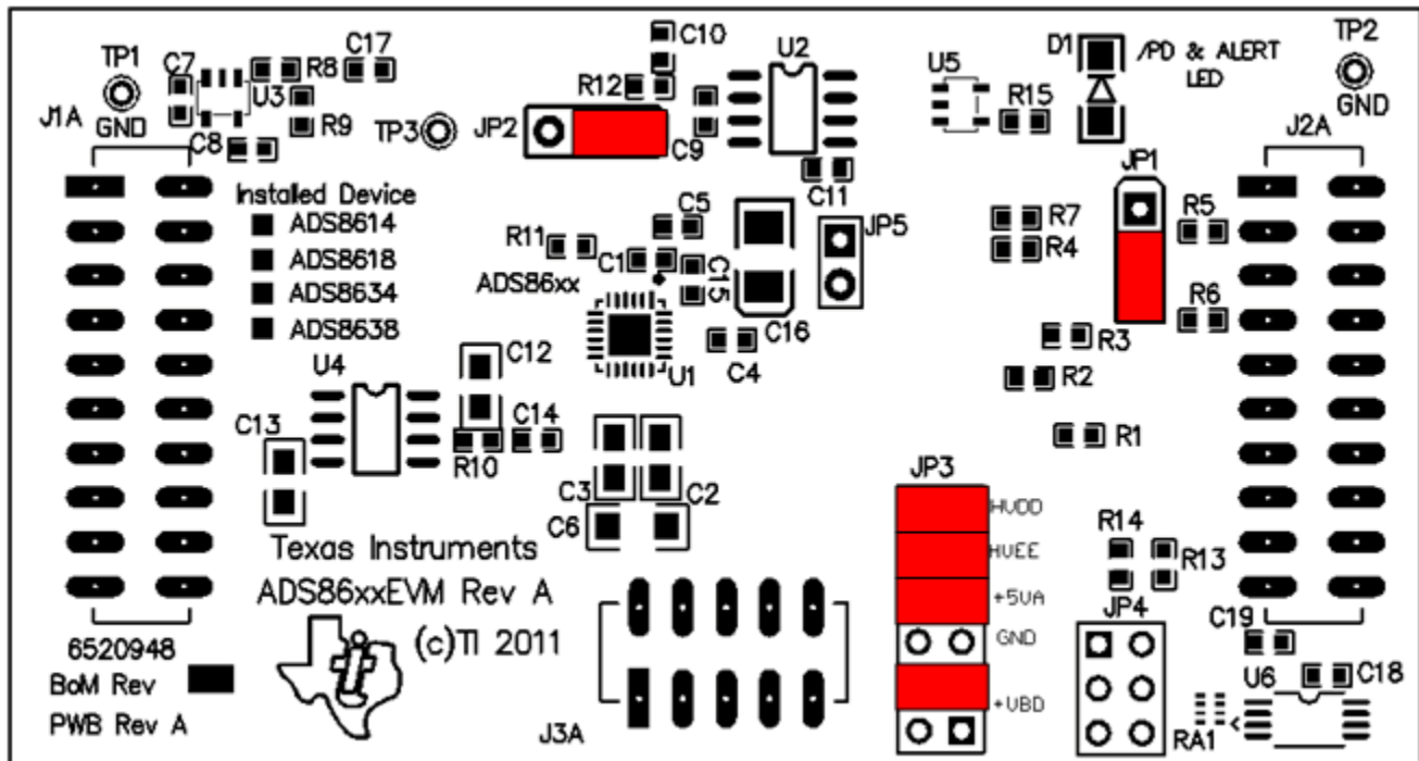
Figure 1. ADS8638EVM Default Jumper Locations
