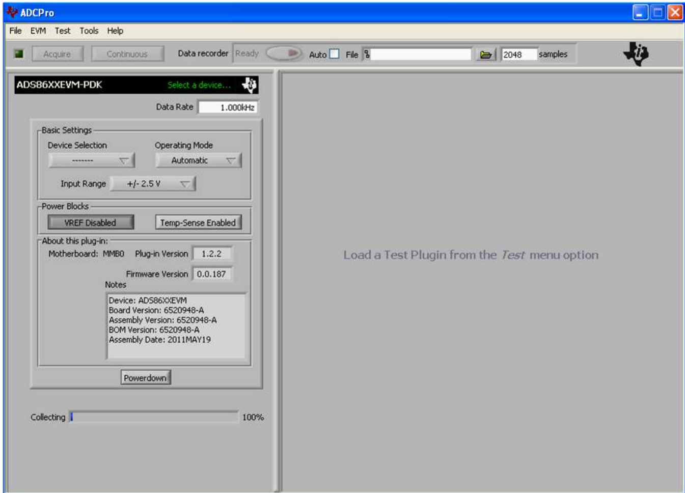
Figure 8. ADS86xxEVM-PDK Plug-in
