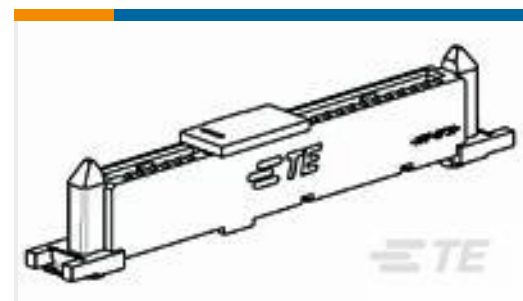
TE Part #1-178128-4 Receptacle and Tab Housing: 5.08 mm Pitch, 250-600V
