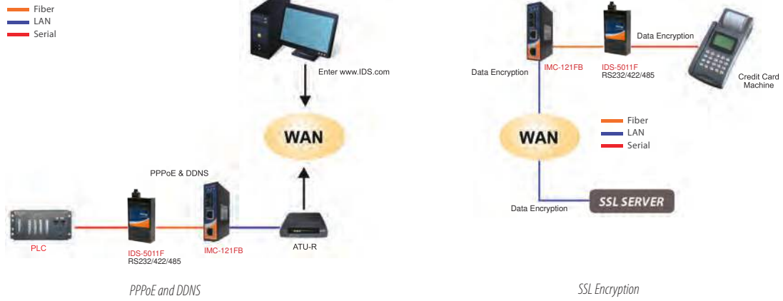
PPPoE and DDNS
