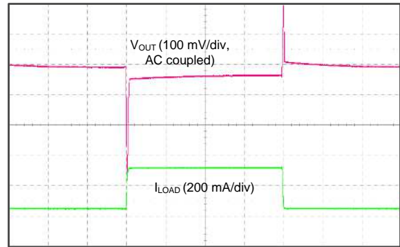
Figure 26. 1.0 V, 50-mA to 300-mA Load Transient
