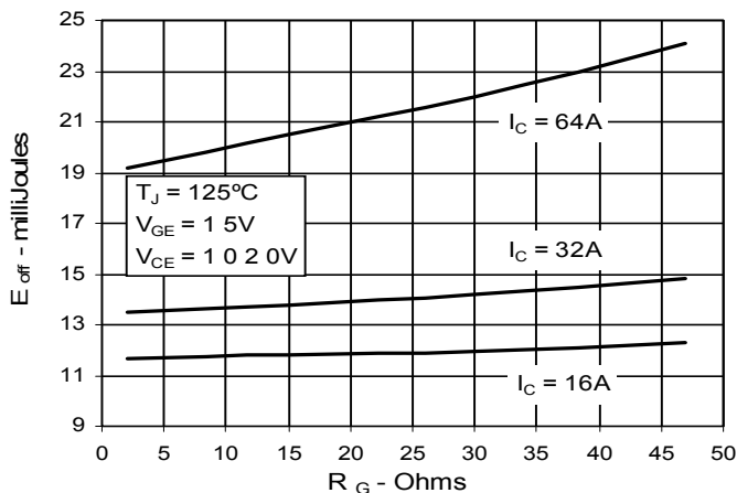
Fig. 10. Dependence of E_{off} on R_G
