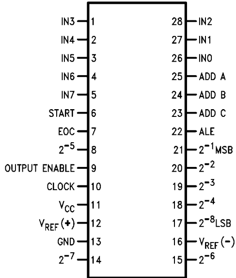
Dual-In-Line Package
