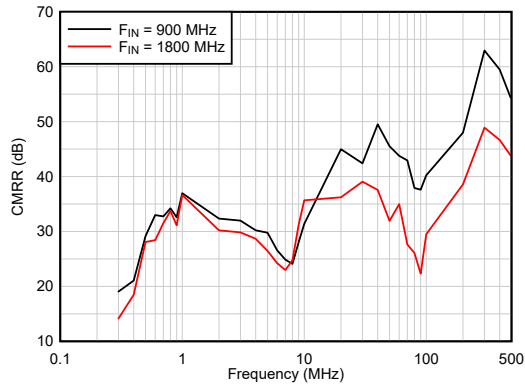
Figure 6-43. CMRR
