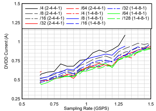
Figure 6-44. Current vs Sampling Rate vs Averaging
