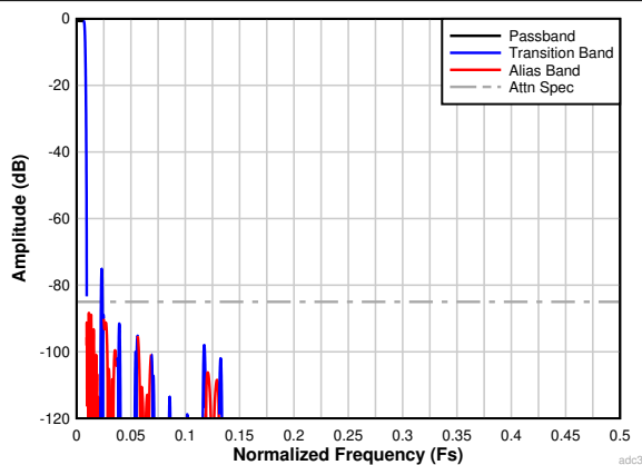
Figure 7-29. Complex Decimation by 64 Filter Response
