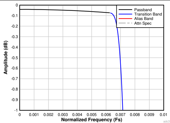
Figure 7-31. Decimation by 64 Passband Ripple Response
