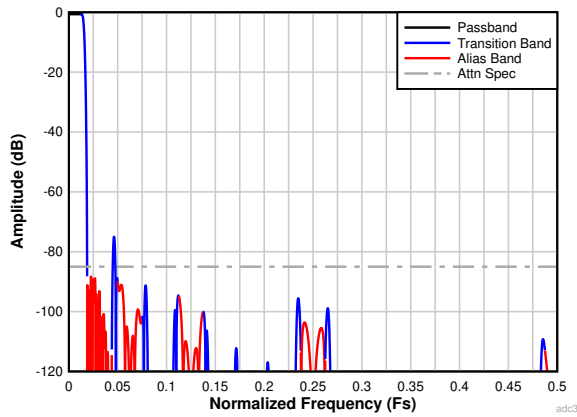
Figure 7-27. Complex Decimation by 32 Filter Response
