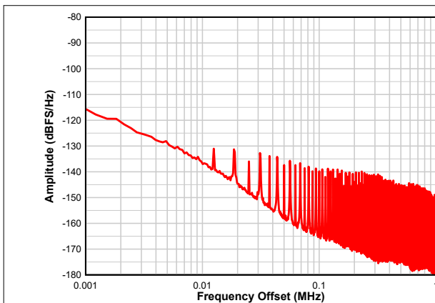
Figure 7-6. Dither Close-Up
