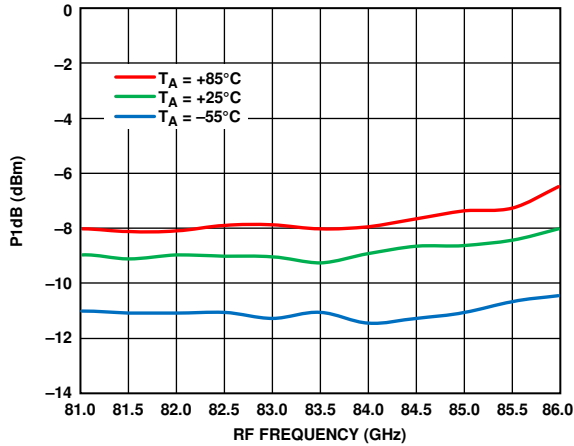
Figure 33. Input P1dB vs. RF Frequency at Various Temperatures, LO = 2 dBm, IF = 500 MHz, V DLNA = 4 V
