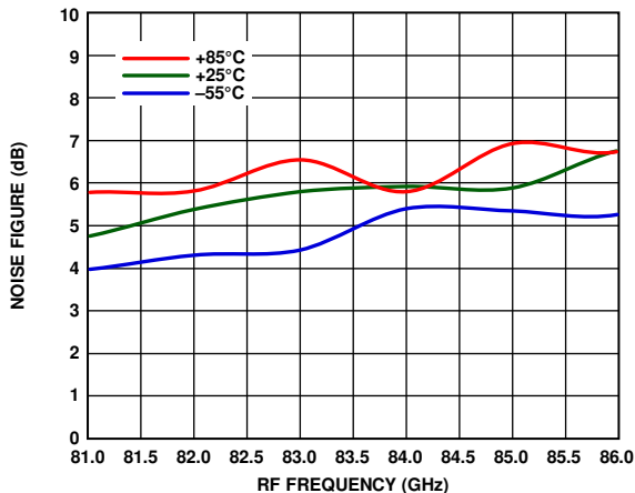
Figure 194. Noise Figure vs. RF Frequency at Various Temperatures, LO = 2 dBm, IF = 2000 MHz, V_{DLNA} = 3 V
