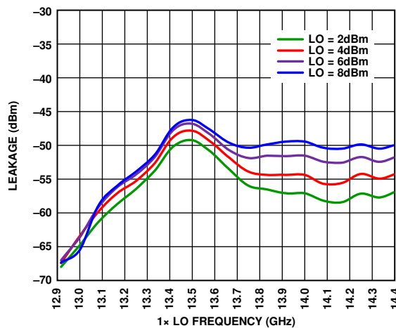
Figure 35. 1x LO Leakage at IFOUT vs. 1x LO Frequency at Various LO Powers, V DLNA = 3 V
