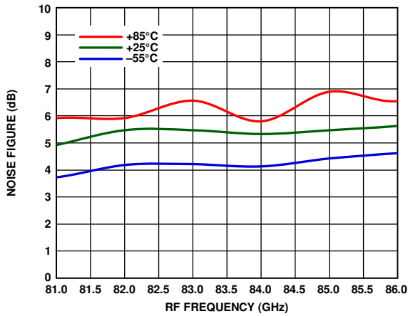
Figure 192. Noise Figure vs. RF Frequency at Various Temperatures, LO = 2 dBm, IF = 500 MHz, V_{DLNA} = 3 V
