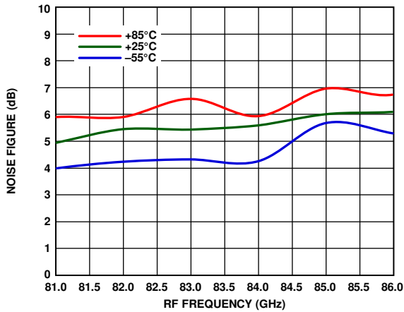
Figure 193. Noise Figure vs. RF Frequency at Various Temperatures, LO = 2 dBm, IF = 1000 MHz, V_{DLNA} = 3 V
