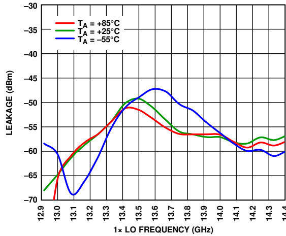
Figure 34. 1x LO Leakage at IFOUT vs. 1x LO Frequency at Various Temperatures, LO = 2 dBm, V DLNA = 3 V
