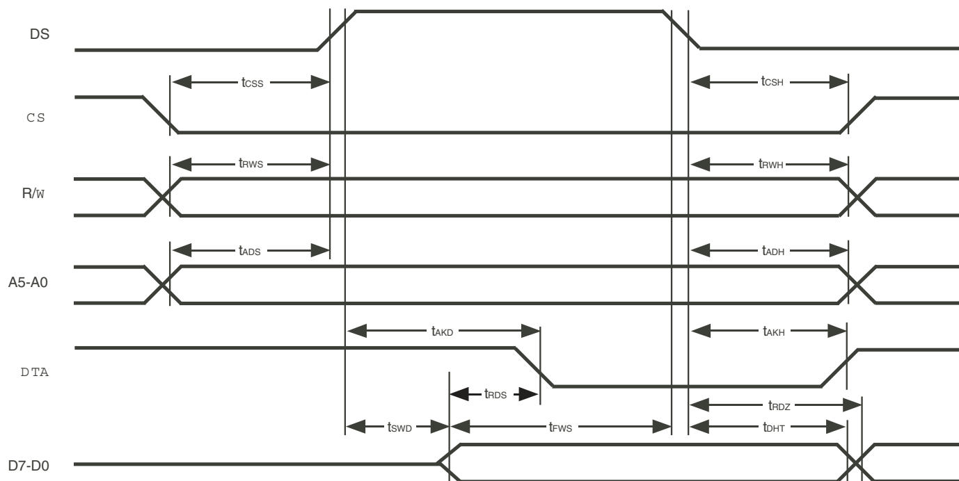
Figure 11. Processor Bus
