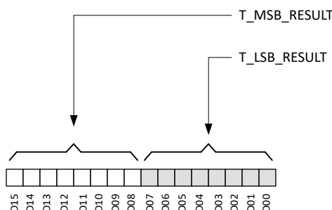
Figure 7-16. Temperature Sensor Data Definition
