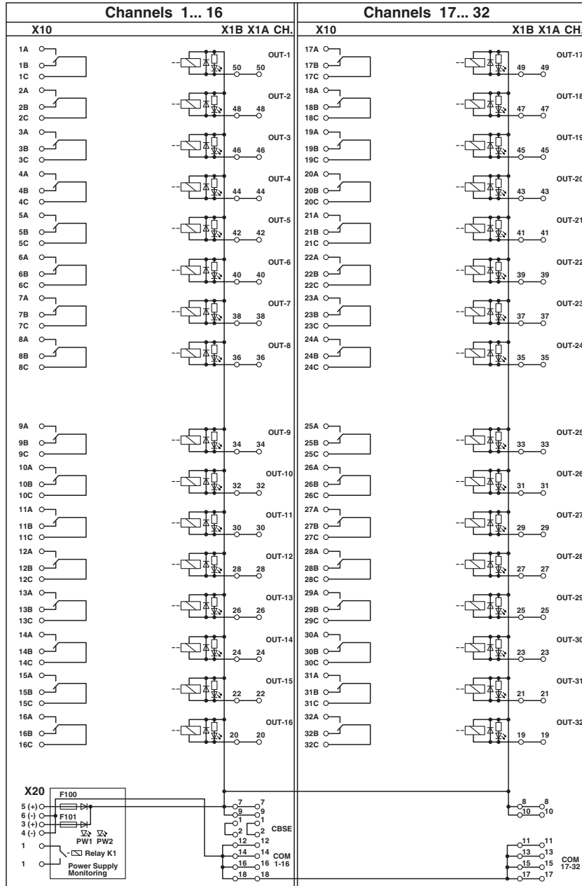
Circuit diagram
