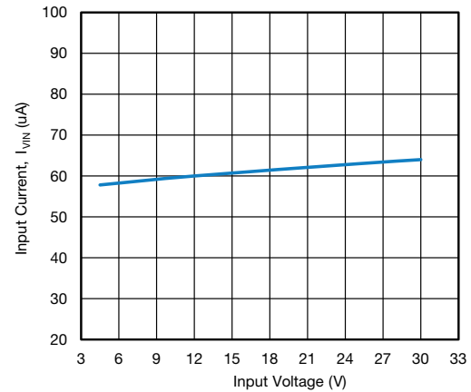
Fig. 38 - Input Current vs. Input Voltage
