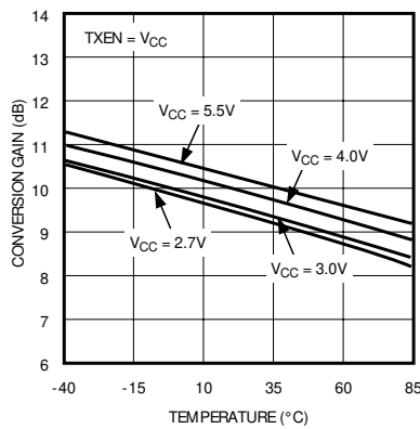
TRANSMIT MIXER CONVERSION GAIN vs. TEMPERATURE
