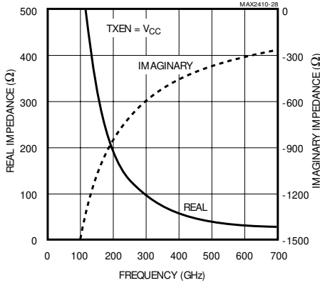
IF INPUT IMPEDANCE vs. FREQUENCY
