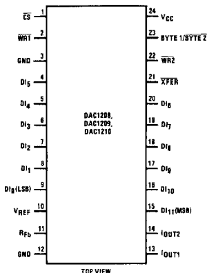
Dual-In-Line Package
