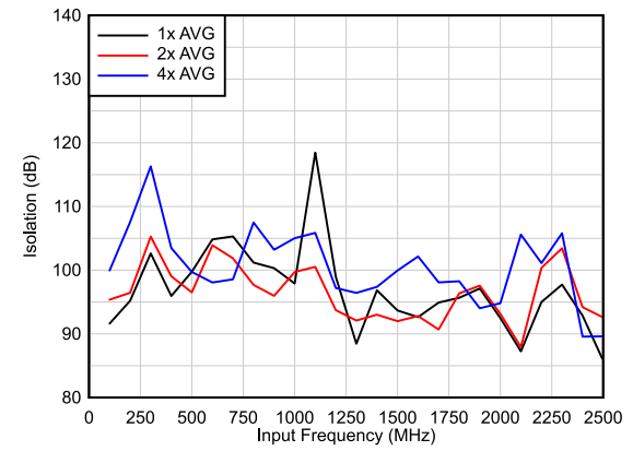
Figure 6-40. Isolation vs Input Frequency
