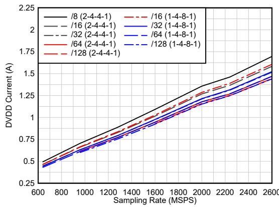
Figure 6-45. Current vs Sampling Rate vs Averaging
