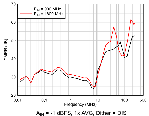
Figure 6-44. CMRR
