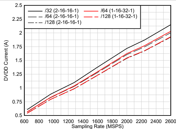
A_{IN} = -1\text{ dBFS} , 1x AVG, Dither = DIS Quad Band Decimation
