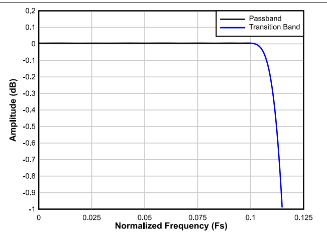
Figure 7-25. Decimation by 4 Passband Ripple Response
