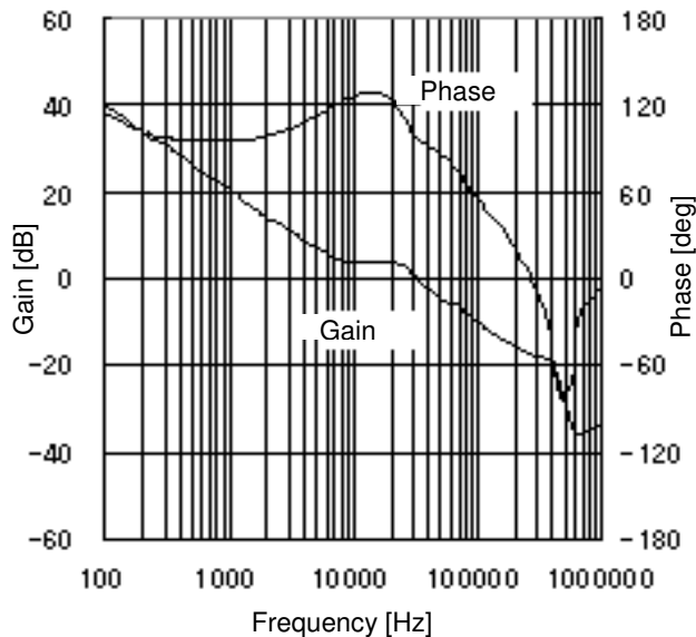
Figure 26 Gain vs Frequency 2 ( V_{CC}=6.0V, I_o=250mA )
