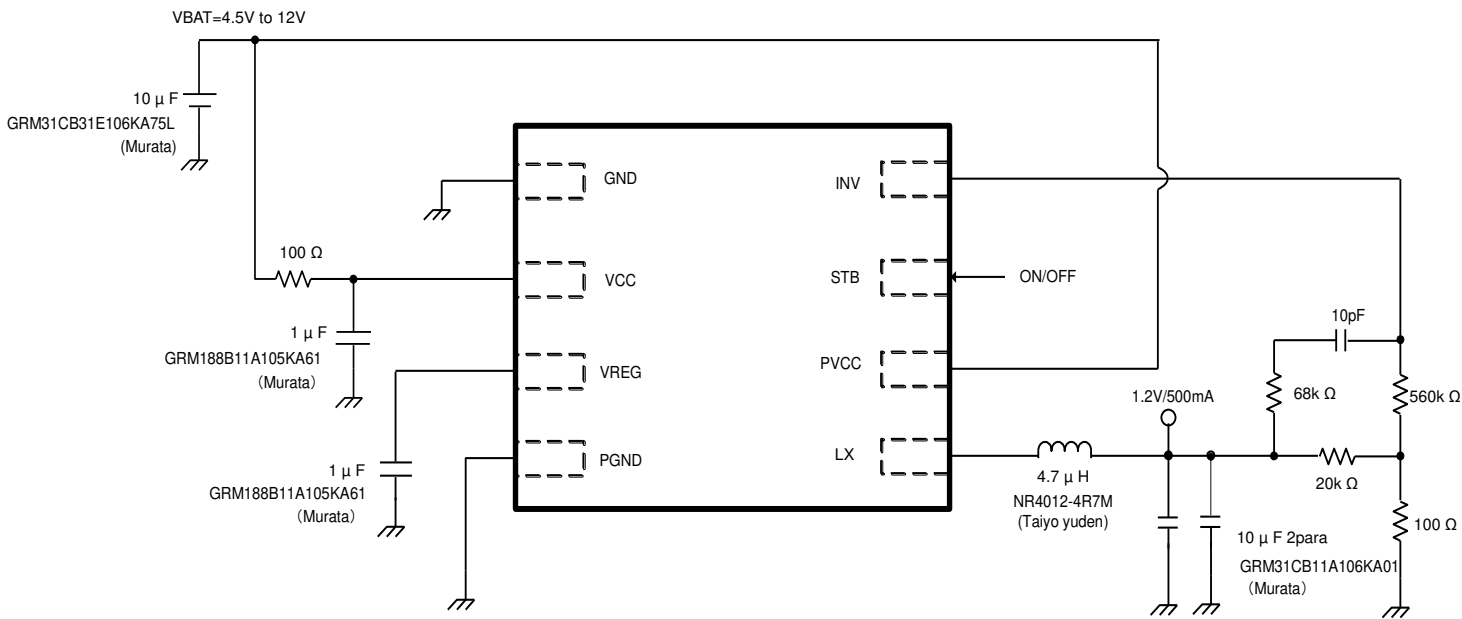
Figure 33. Reference Application Diagram 2
