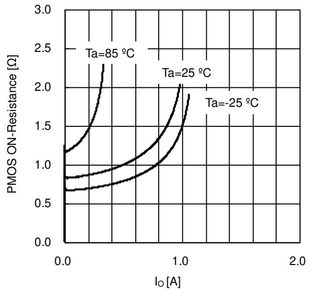
Figure 15. Pch FET ON-Resistance vs I_O ( V_{CC} = 3.5\text{V} )
