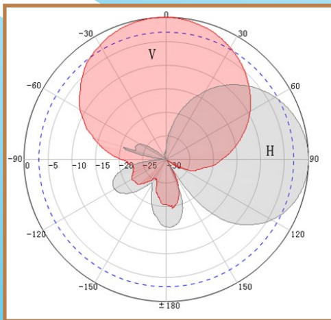
Radiation Pattern 915 MHz
